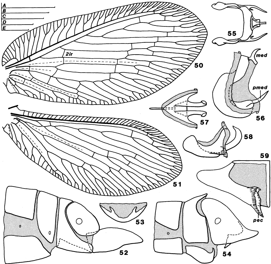
Figs. 50–59. Wesmaelius concinnus . 50, Forewing [Scale bar B]. 51, Hind wing [B]. 52, Female terminalia, lateral [D]. 53, Male 9th sternite, posterior [D]. 54, Male terminalia, lateral [D]. 55, Gonarcus, dorsal [C]. 56, Gonarcus, lateral [C]. 57, Parabaculum, dorsal [A]. 58, Parabaculum, lateral [A]. 59, Ventrodistal portion of male ectoproct, mesal [E]. Abbreviations: 2ir, 2nd series intraradial crossvein; med, mediuncus; pec, pecten; pmed, paramediuncus. Scale bars (mm): A = 0.5; B = 2.0; C = 0.5; D = 0.5; E = 0.2.
