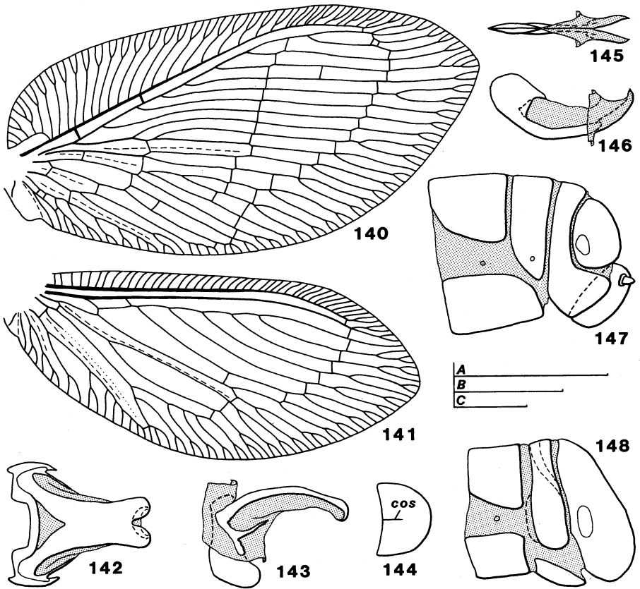
Figs. 140–148. Austromegalomus insulanus . 140, Forewing [Scale bar A]. 141, Hind wing [A]. 142, Gonarcus, dorsal [C]. 143, Gonarcus, lateral [C]. 144, Male 9th sternite, dorsal [B]. 145, Parabaculum, dorsal [C]. 146, Parabaculum, lateral [C]. 147, Female terminalia, lateral [B]. 148, Male terminalia, lateral [B]. Abbreviations: cos, costa. Scale bars (mm): A = 2.0; B = 0.5; C = 0.2.
