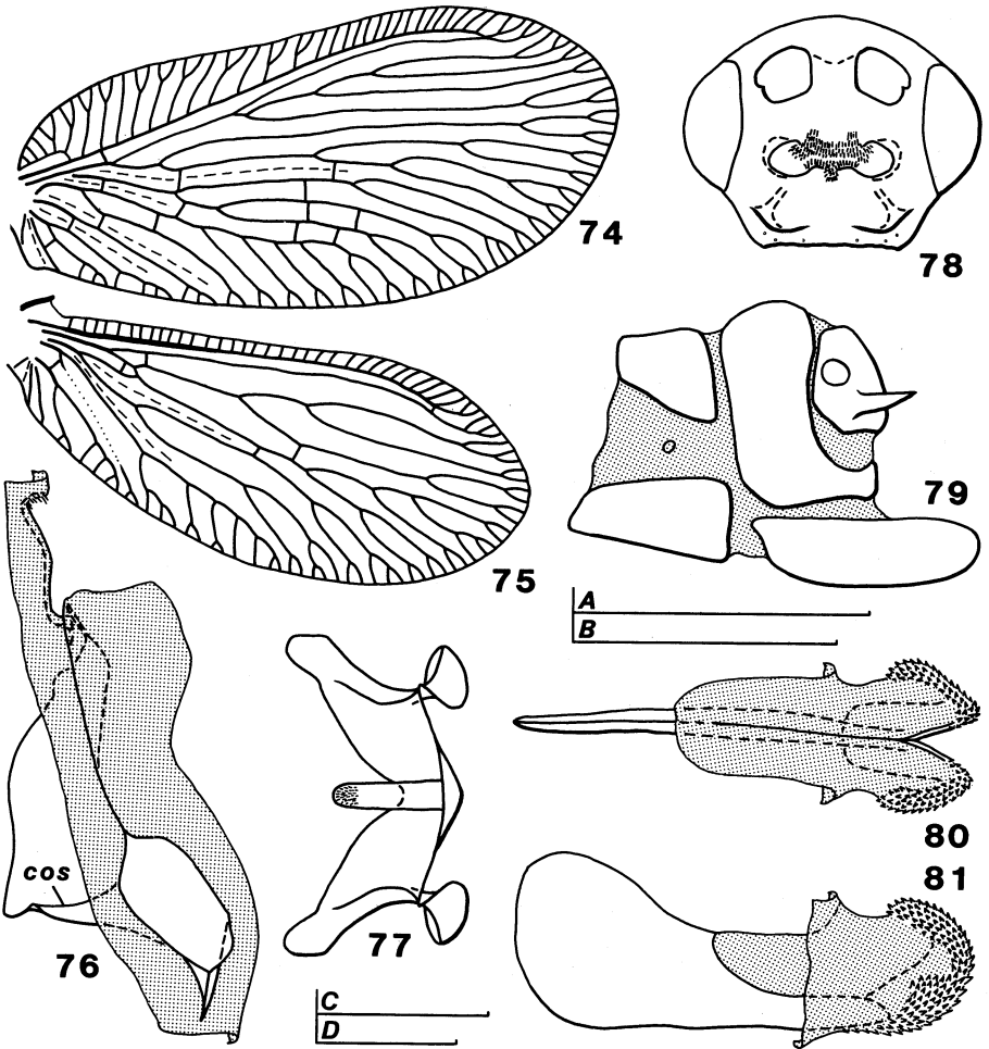
Figs. 74–81. Neosymphorobius cinereus . 74, Forewing [Scale bar A]. 75, Hind wing [A]. 76, Gonarcus, lateral [D]. 77, Gonarcus, dorsal [D]. 78, Cranium, anterior [C]. 79, Male terminally, lateral [B]. 80, Parabaculum, dorsal [D]. 81, Parabaculum, lateral [D]. Abbreviations: cos, costa. Scale bars (mm): A = 2.0; B = 0.5; C = 0.5; D = 0.1.
