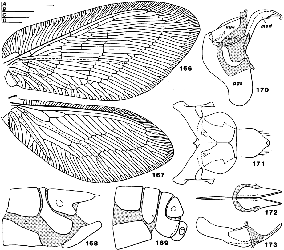
Figs. 166–173. Neuronema decisum (except as noted). 166, Forewing [Scale bar C]. 167, Hind wing [C]. 168, Male terminalia, lateral [D]. 169, Female terminalia ( kuwayamai ), lateral [D]. 170, Gonarcus, lateral [A]. 171, Gonarcus, dorsal [A]. 172, Parabaculum, dorsal [B]. 173, Parabaculum, lateral [B]. Abbreviations: med, mediuncus; ngs, neogonarcus; pgs, paleogonarcus. Scale bars (mm): A = 0.5; B = 0.5; C = 2.0; D = 0.5.
