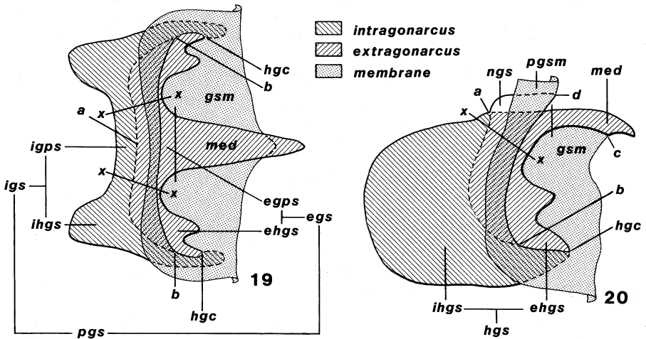
Figs. 19–20. Male gonarcus terminology. 19, Gonarcus, dorsal (diagrammatic). 20, Gonarcus, lateral (diagrammatic). Abbreviations: a, b, c, d, reference points; egps, extragonopons; egc, extragonarcus; ehgs, extrahemigonarcus; gsm, gonosaccal membrane; hgc, hemigonarcus; hgs, hemigonarcus; igps, intragonopons; igs, intragonarcus; ihgs, intrahemigonarcus; med, mediuncus; ngs, neogonarcus; pgs, paleogonarcus; pgsm, paragonosaccal membrane; x-x, reference line.
